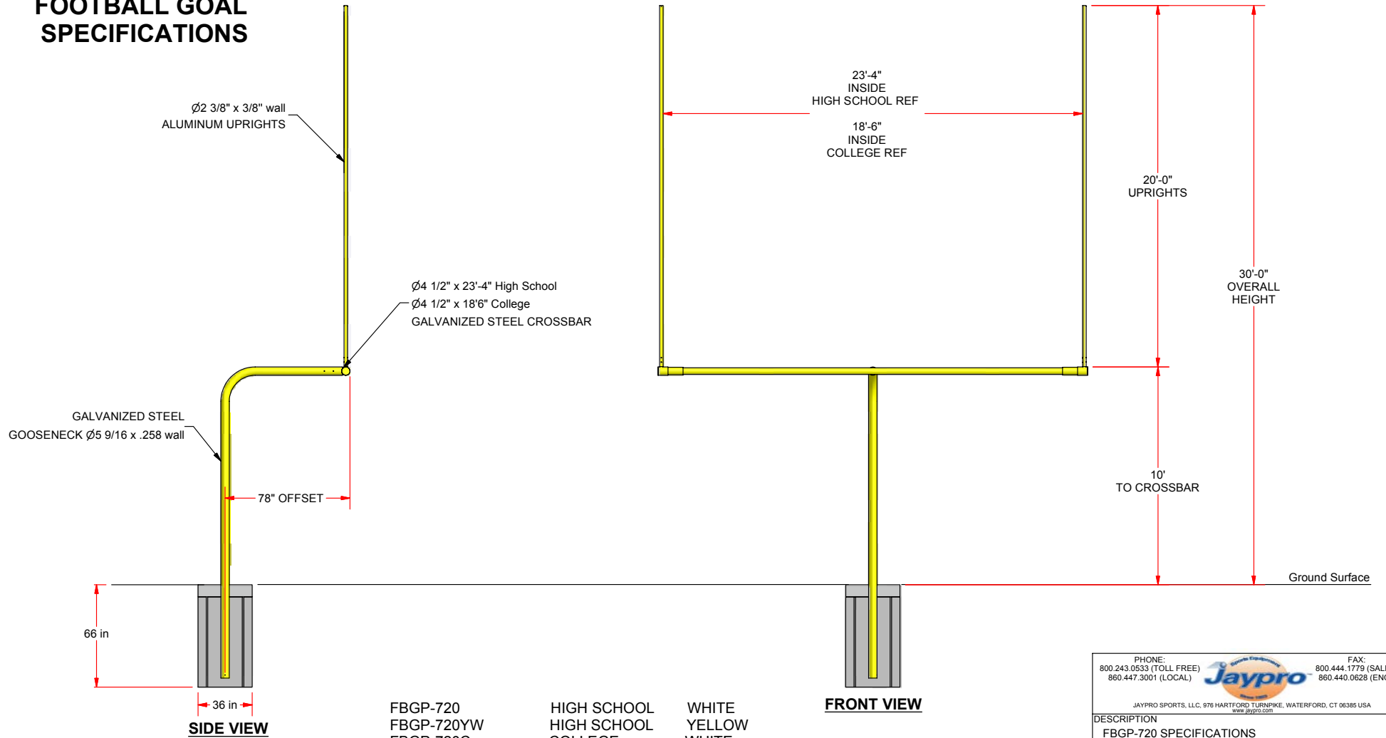
SIDE VIEW
