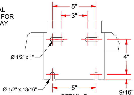
DETAIL B MOUNTING PATTERN
