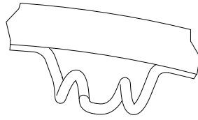
DETAIL A TYPICAL PIG TAIL NET ATTACHMENT SYSTEM (12 PLACES)
